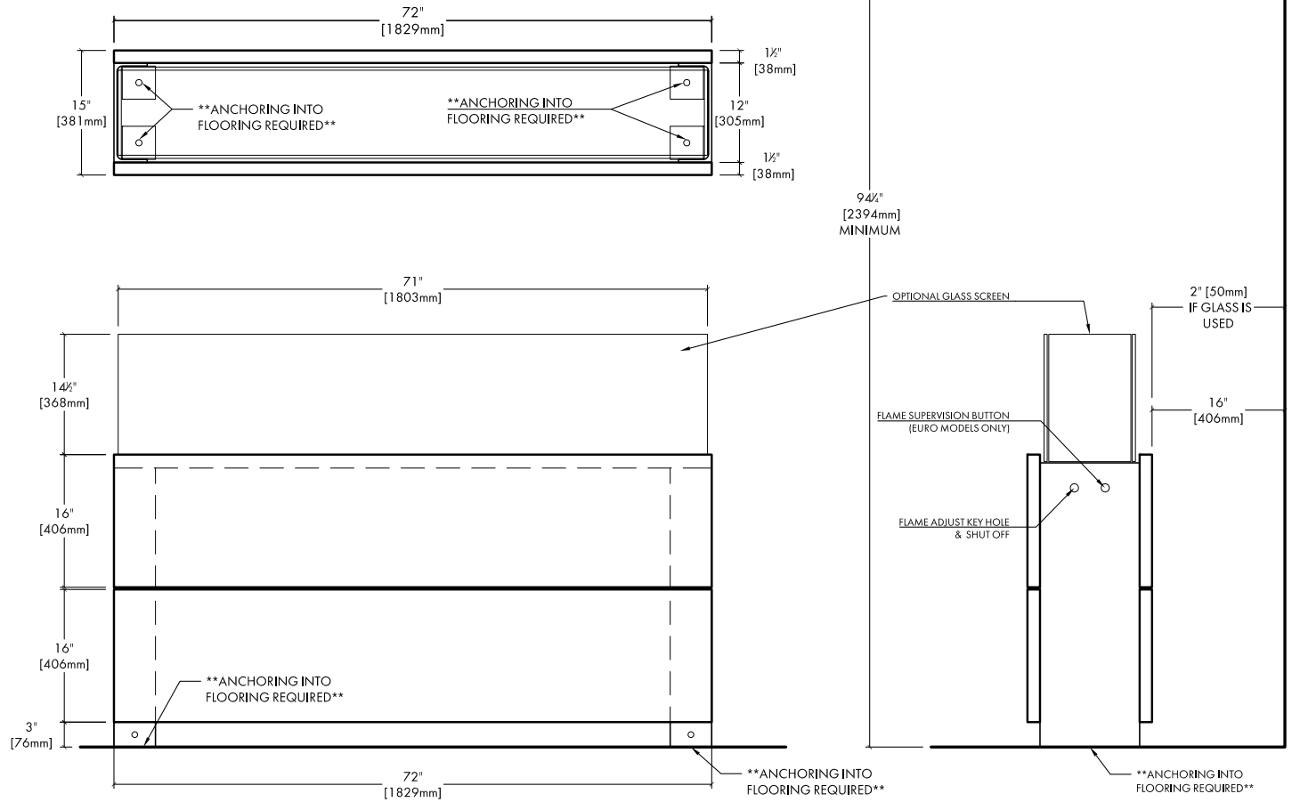
CLEARANCES to ADJACENT MATERIALS
